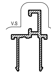
AS7 45mm DOOR STOP Mass. 0.269 Kg/m Anod. Per. 154 Paint Per. 100
