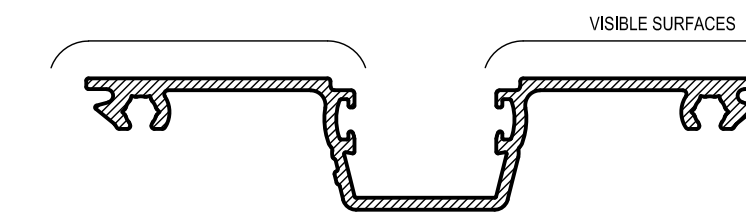
ME4 GLAZING ADAPTOR Mass. 0.685 Kg/m Anod. Per. 303 Paint Per. 100 lxx = 187.7 x 10 3 mm 4
