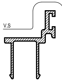
AS36 ALTERNATE 35mm DOOR STOP Mass. 0.297 Kg/m Anod. Per. 157 Paint Per. 100
