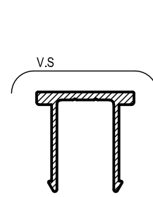
AS8 POCKET FILLER Mass. 0.186 Kg/m Anod. Per. 109 Paint Per. 100
