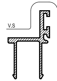
AS30 35mm OFFSET DOOR STOP Mass. 0.279 Kg/m Anod. Per. 152 Paint Per. 100
