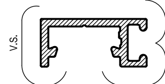
AS9 CONCEALED PLANT ON DOOR STOP Mass. 0.315 Kg/m Anod. Per. 125 Paint Per. 100
