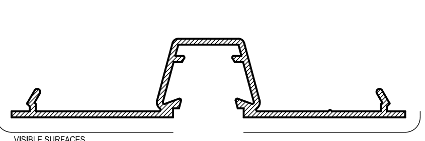
PB66 GLAZING ADAPTOR Mass. 0.741 Kg/m Anod. Per. 332 Paint Per. 100
