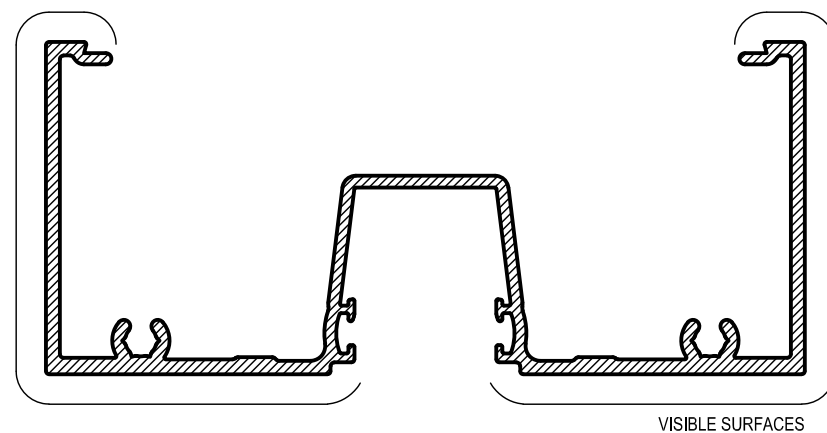
ME1 FRAME / JAMB Mass. 1.365 Kg/m Anod. Per. 560 Paint Per. 182 lxx = 695.7 x 10 3 mm 4
