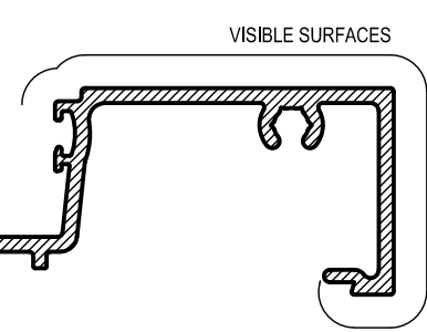
ME52 25mm SILL Mass. 0.931 Kg/m Anod. Per. 379 Paint Per. 100 lxx = 377.6 x 10 3 mm 4 lyy = 25.8 x 10 3 mm 4
