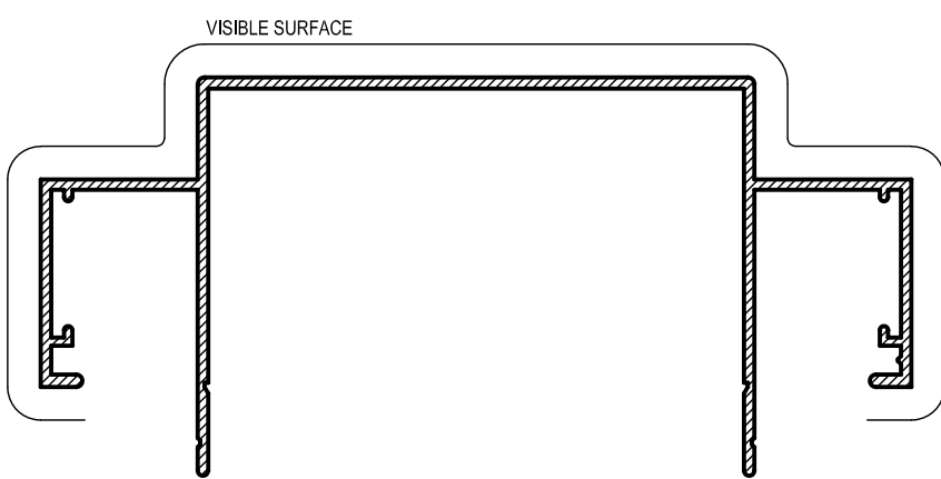
PB65 SHADOW LINE FRAME Mass. 0.902 Kg/m Anod. Per. 526 Paint Per. 190 lxx = 456.92 x 10 3 mm 4 lyy = 64.67 x 10 3 mm 4
