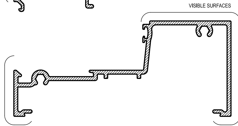
ME3 SILL BEAD Mass. 0.367 Kg/m Anod. Per. 203 Paint Per. 100
