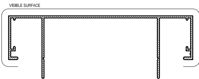
PB60 MAIN FRAME Mass. 0.775 Kg/m Anod. Per. 478 Paint Per. 155 lxx = 411.27 x 10 3 mm 4 lyy = 31.38 x 10 3 mm 4
