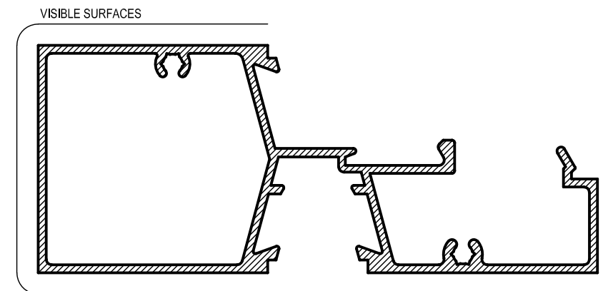
PB67 TRANSOM Mass. 1.506 Kg/m Anod. Per. 646 Paint Per. 190 lxx = 520.10 x 10 3 mm 4 lyy = 118.76 x 10 3 mm 4
