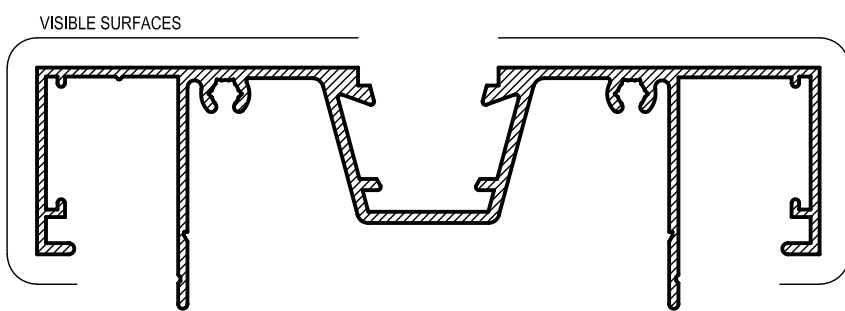
PB64 GLAZING FRAME Mass. 1.100 Kg/m Anod. Per. 586 Paint Per. 137 lxx = 442.89 x 10 3 mm 4 lyy = 32.62 x 10 3 mm 4
