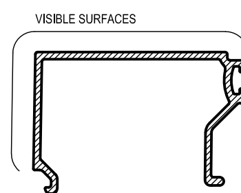
ME3 SILL BEAD Mass. 0.367 Kg/m Anod. Per. 203 Paint Per. 100
